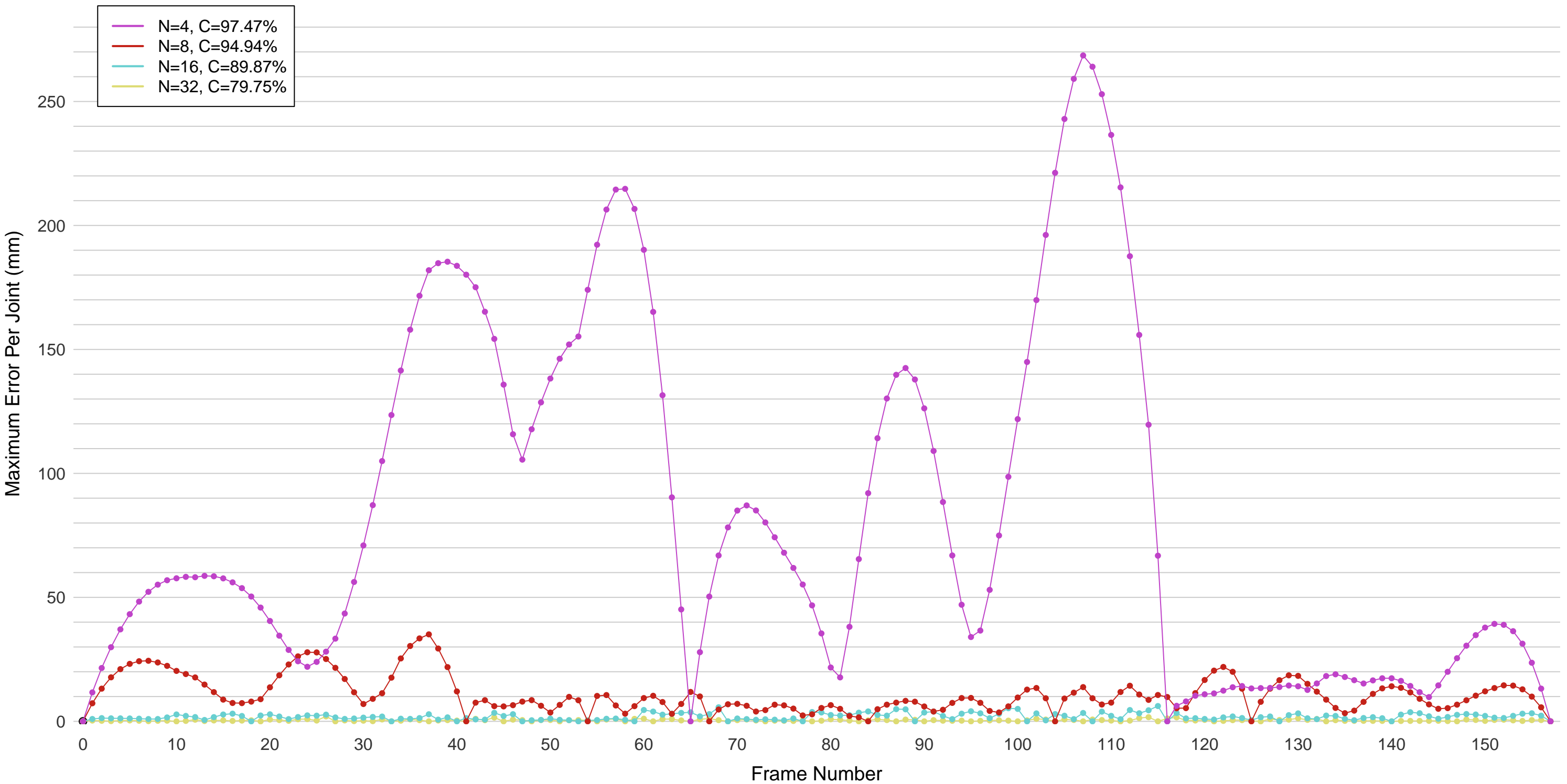
Error Curves at Compression Levels, Baseball Umpire
