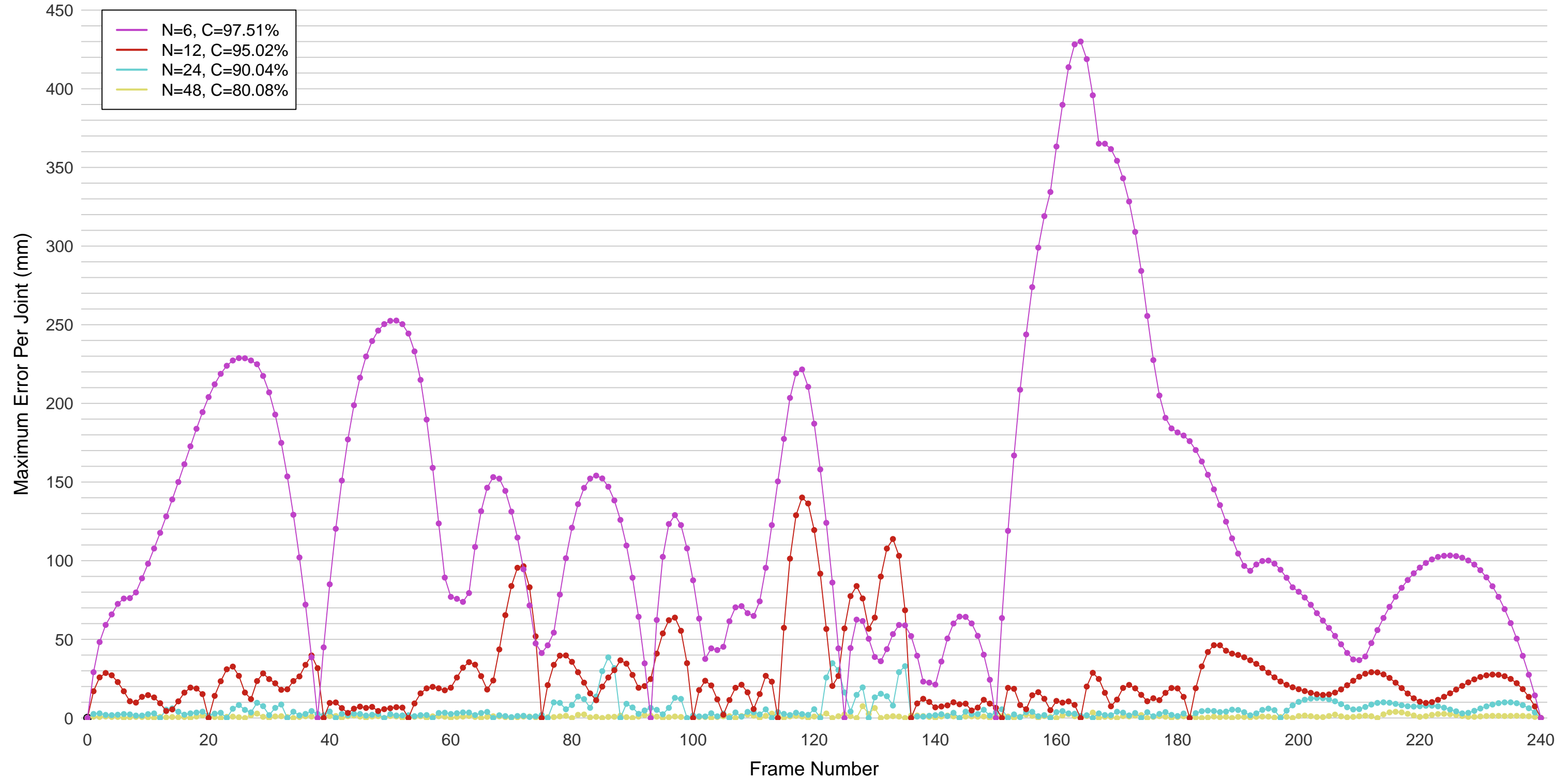
Error Curves at Compression Levels, Climbing To Top
