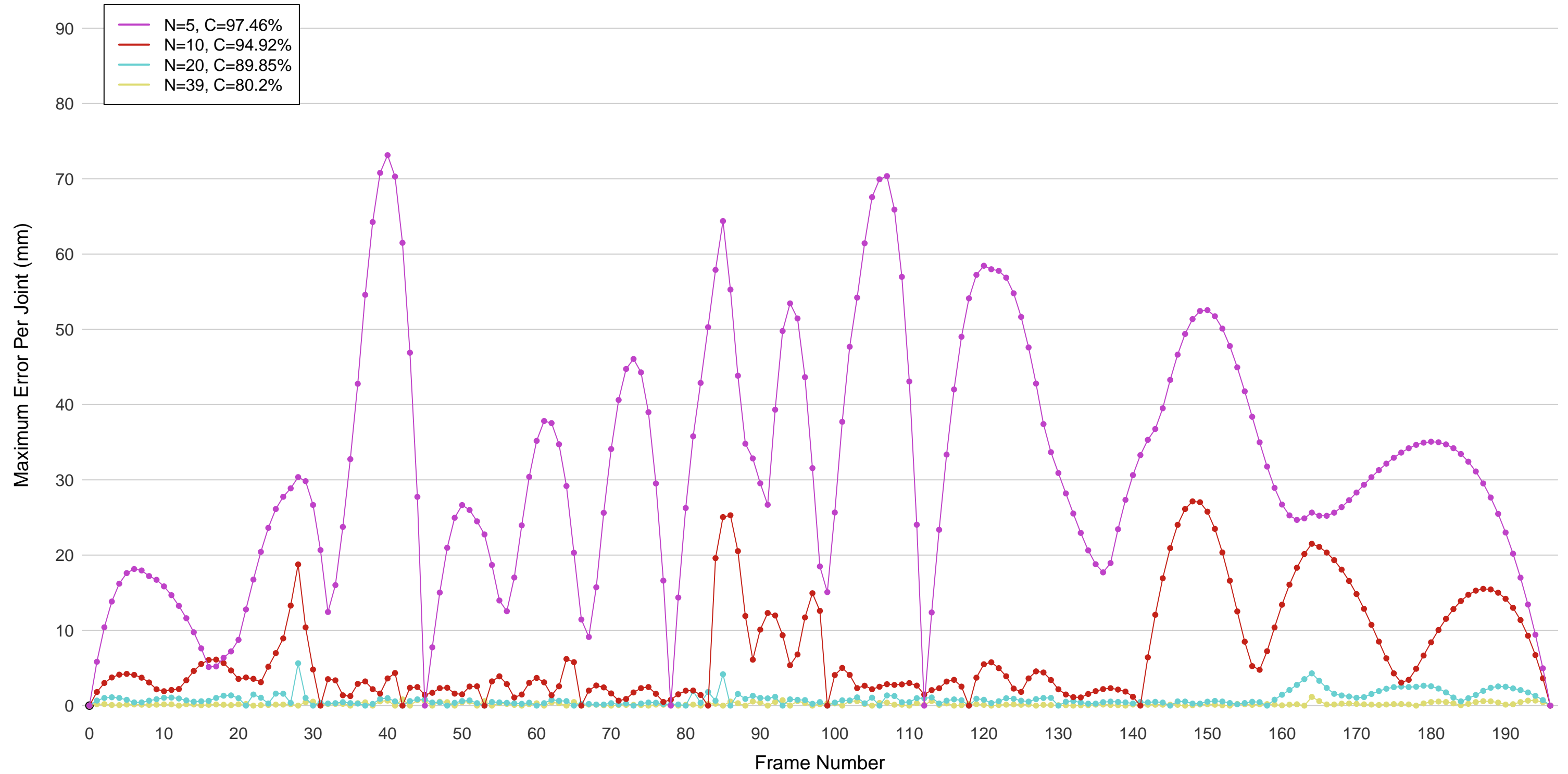
Error Curves at Compression Levels, Football Hike
