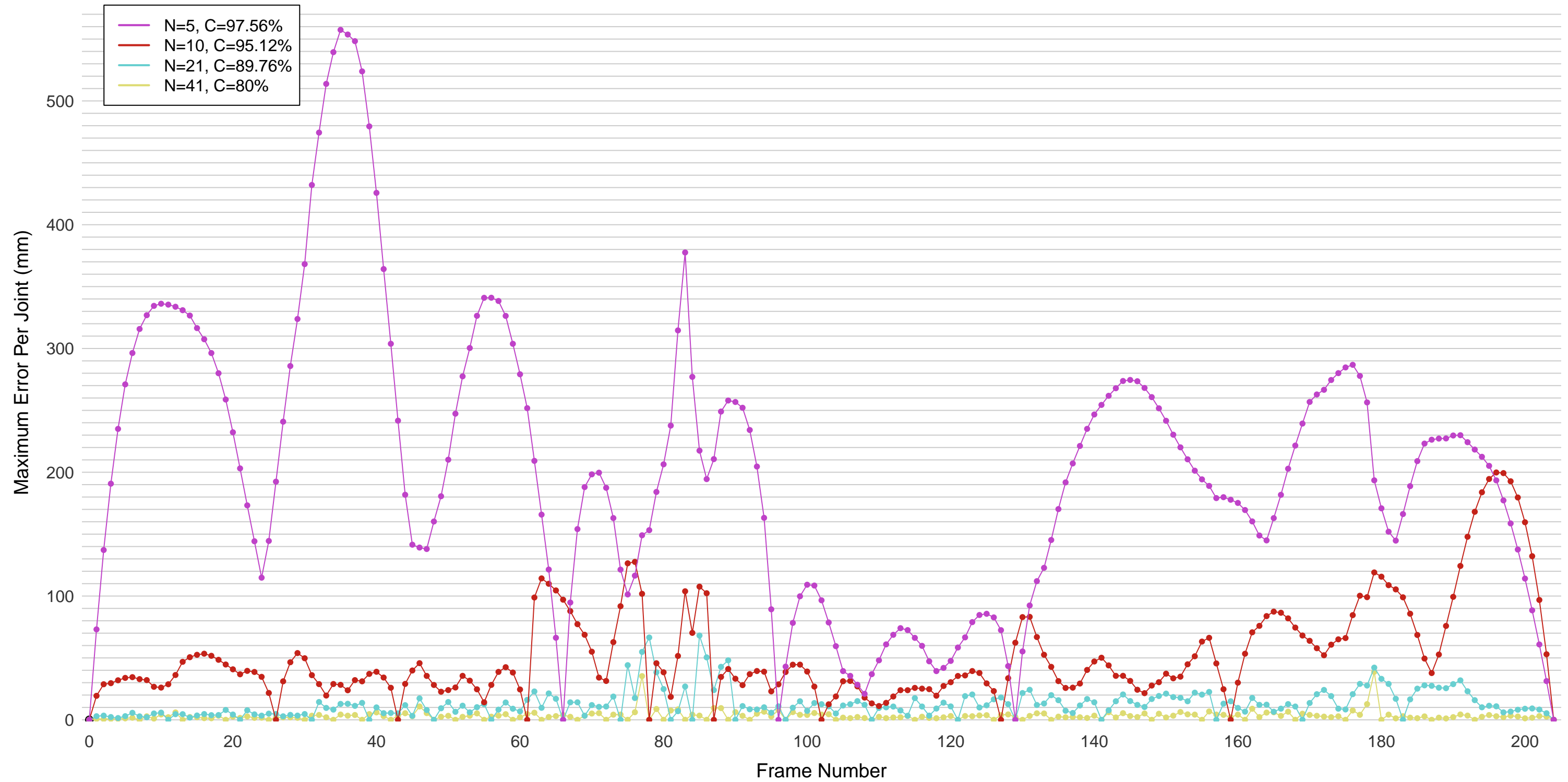
Error Curves at Compression Levels, Goalkeeper Diving Save
