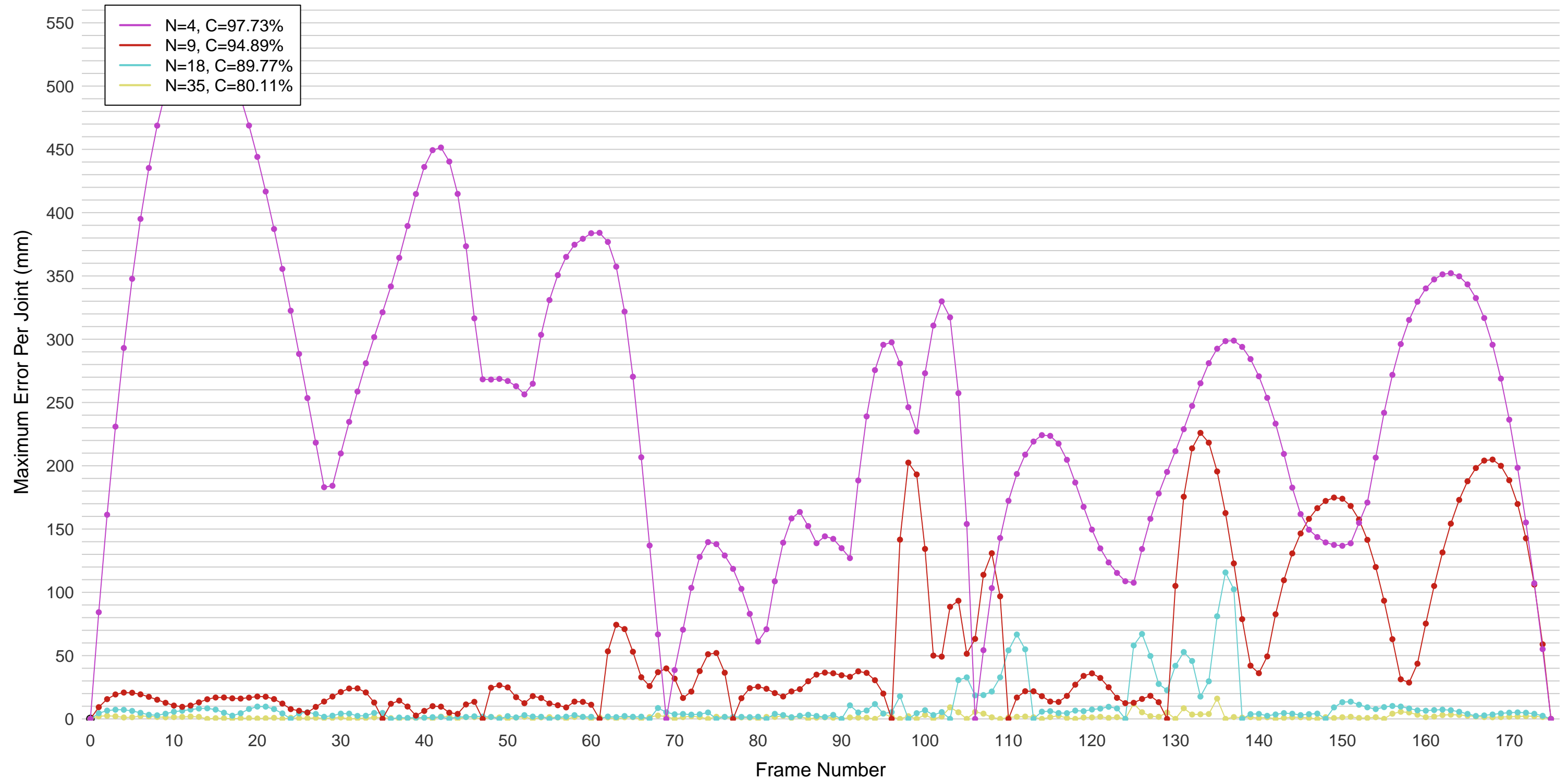
Error Curves at Compression Levels, Jumping Down
