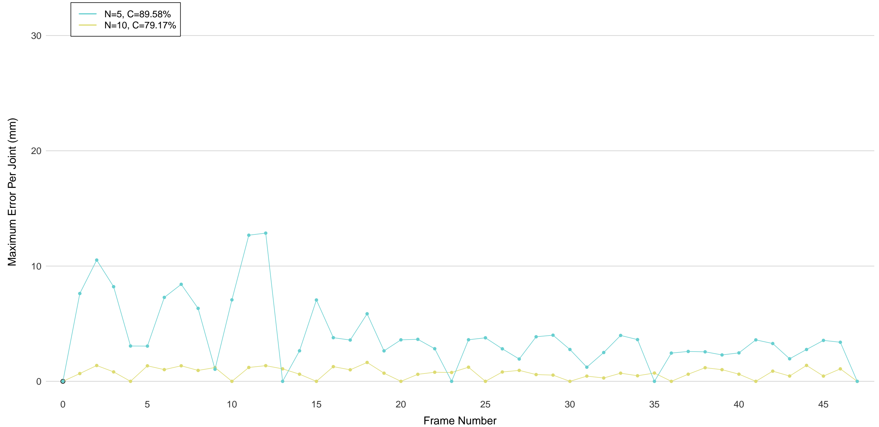
Error Curves at Compression Levels, Long Left Side Step
