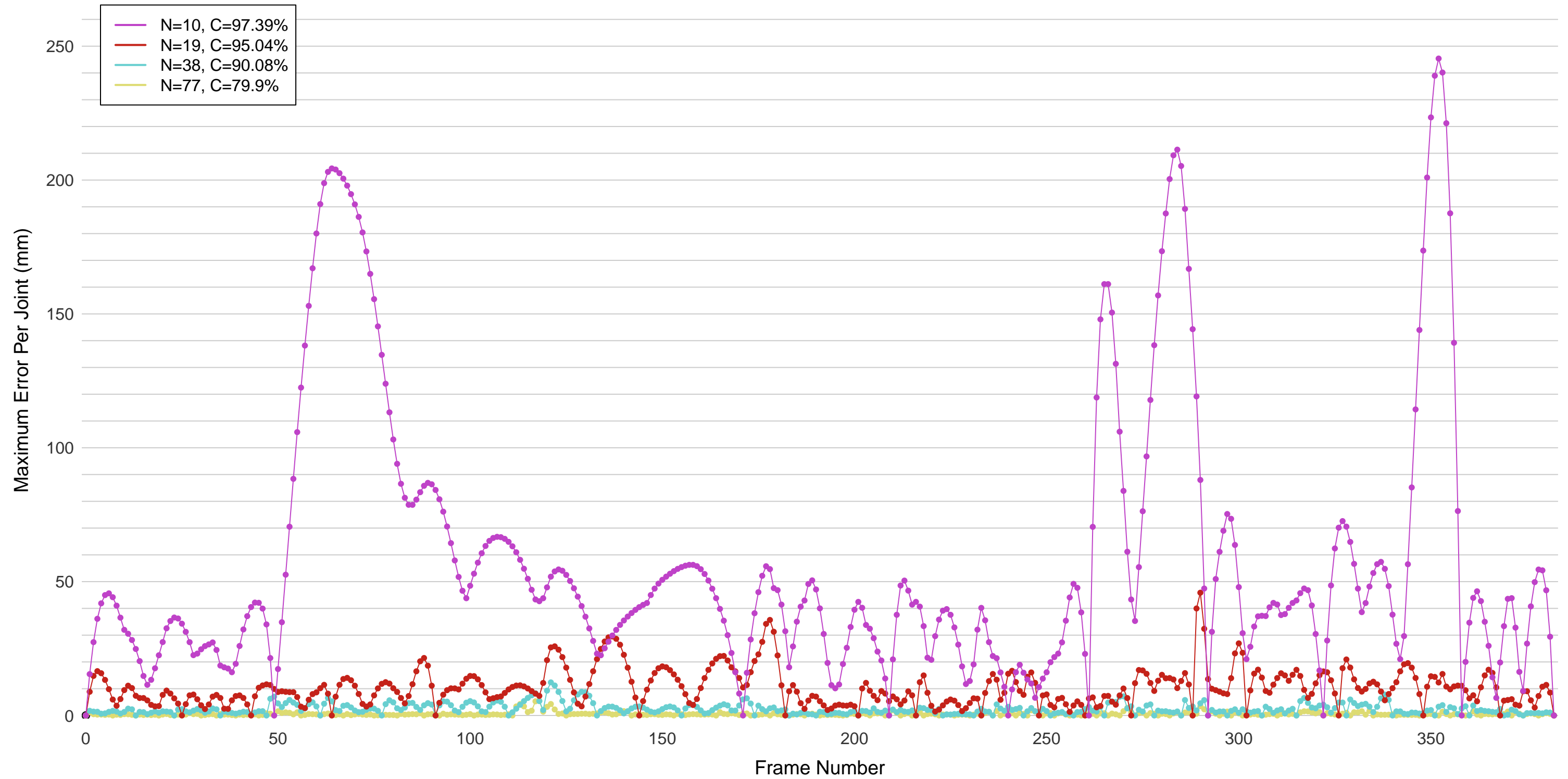
Error Curves at Compression Levels, Opening Door Inwards
