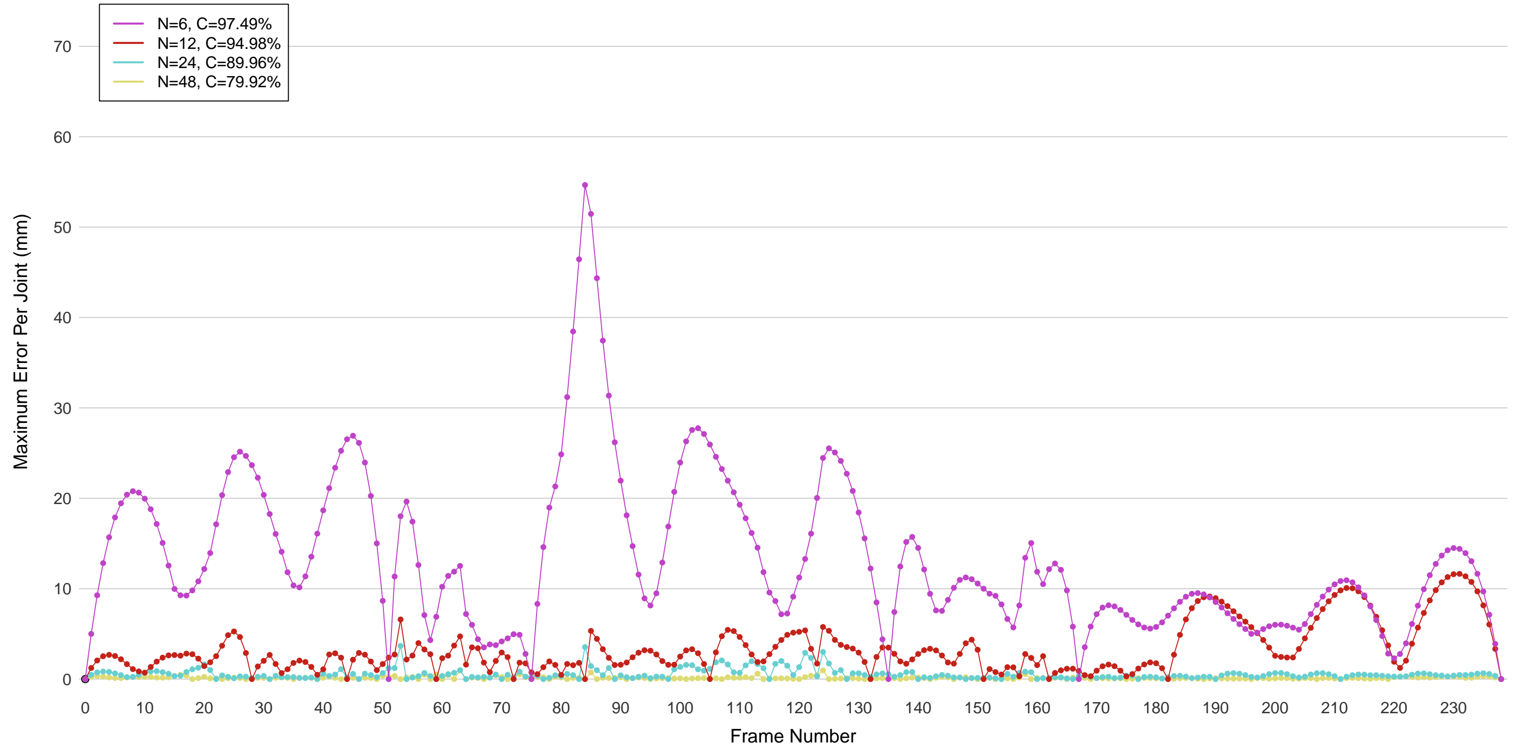
Error Curves at Compression Levels, Put Back Rifle Behind Shoulder
