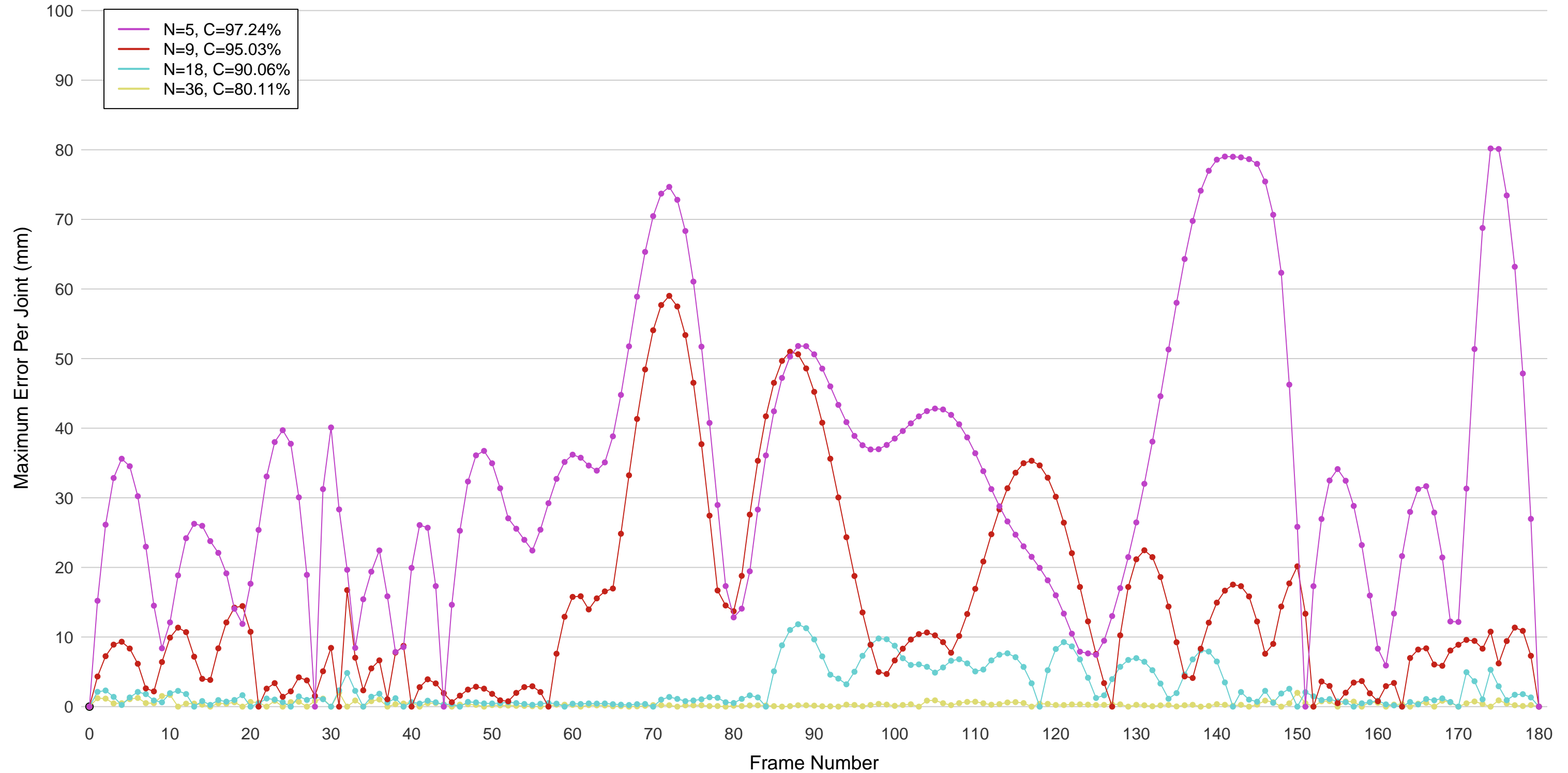
Error Curves at Compression Levels, Reaching Down
