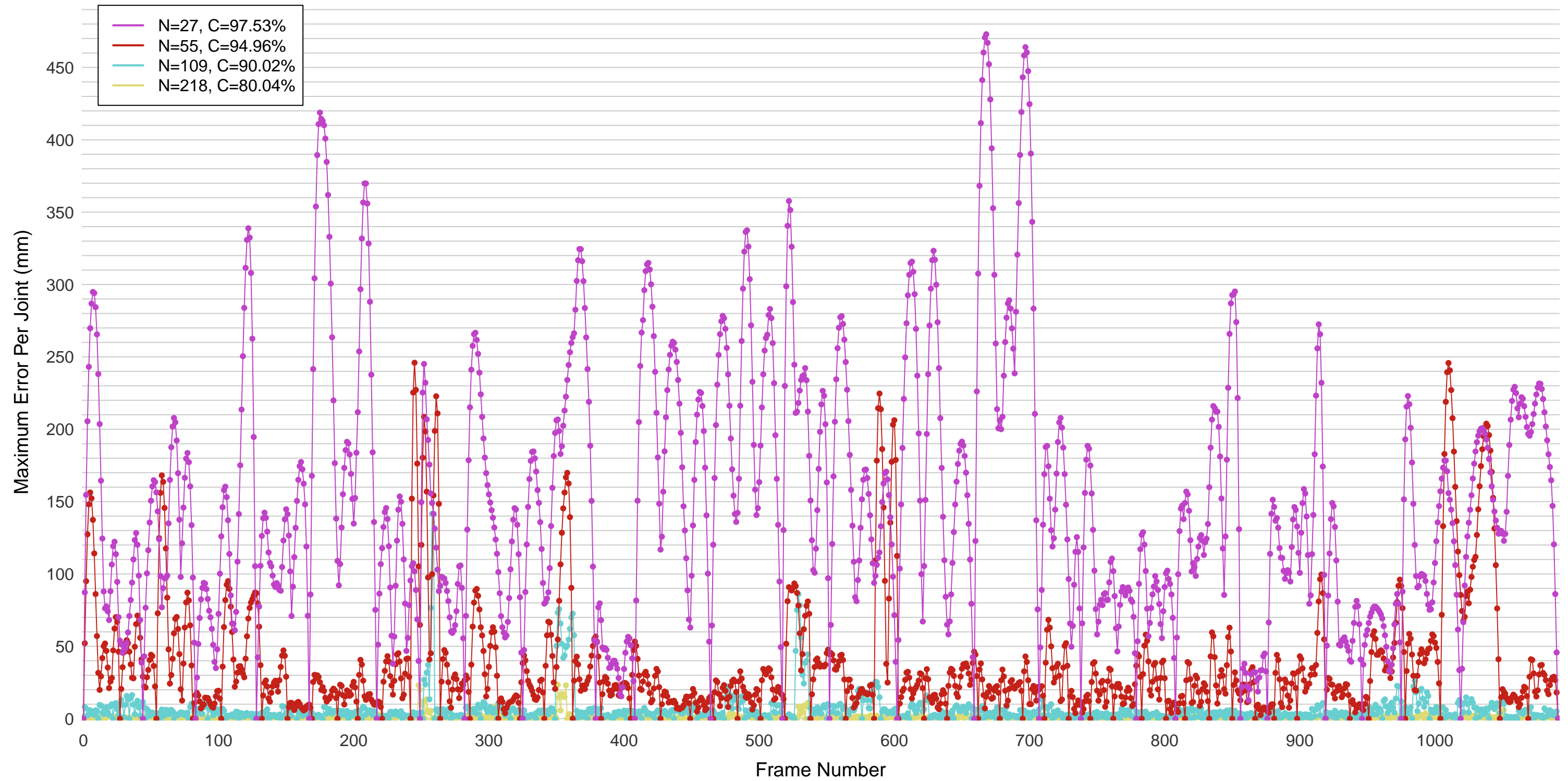
Error Curves at Compression Levels, Samba Dancing
