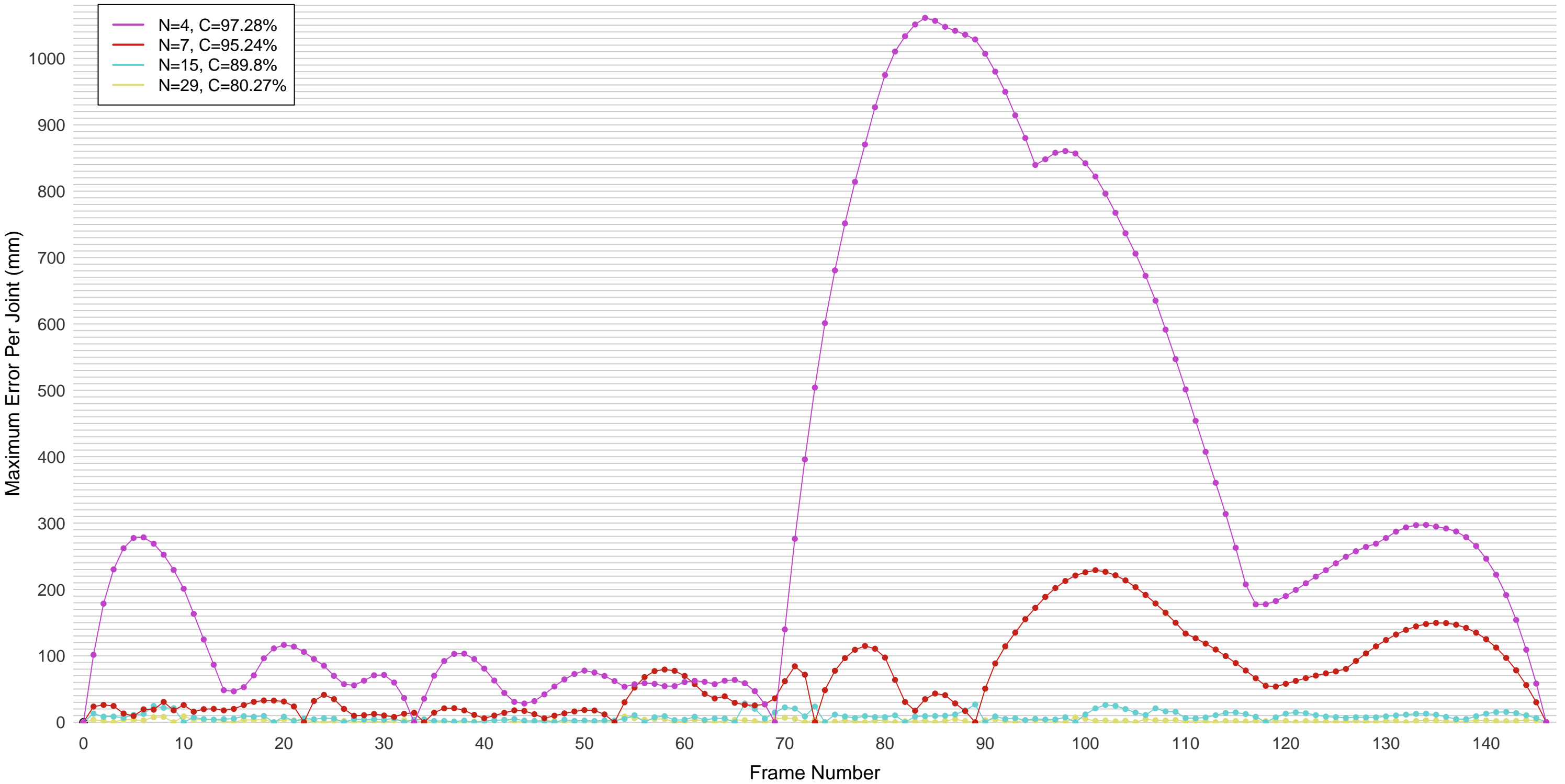
Error Curves at Compression Levels, Swinging
